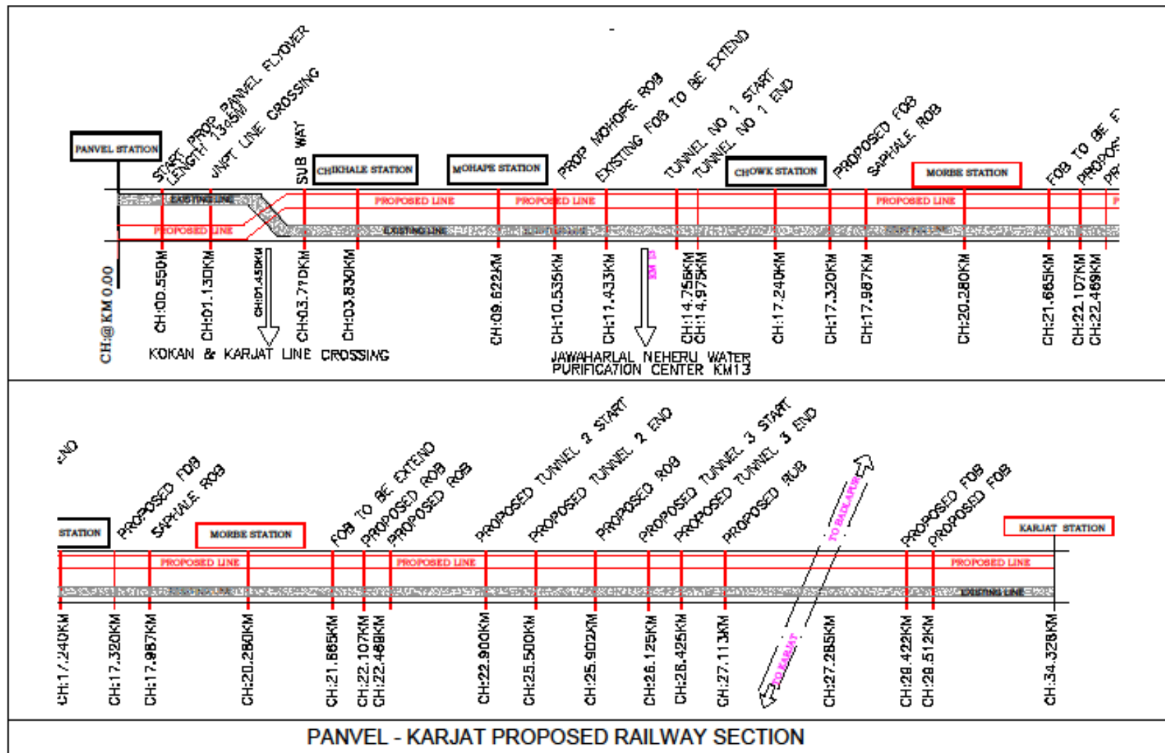
Figure 1.2: Schematic Diagram of Project Components (Not to scale)
